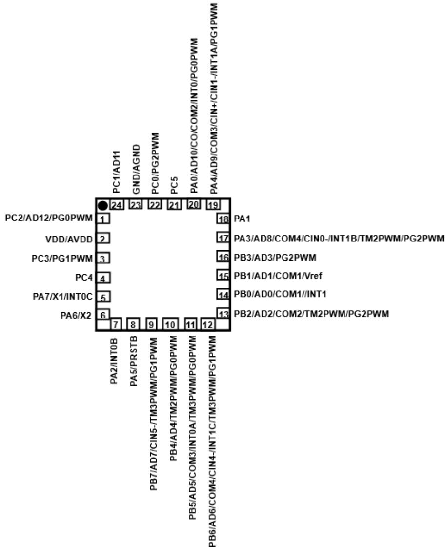
PMS134G-2J24A (QFN4*4-24P-0.5pitch)
