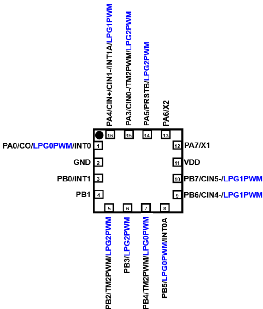
PMS152G-1J16A (QFN3*3-16P-0.5pitch)
