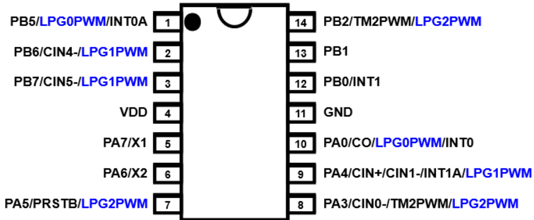
PMS152G-S14 (SOP14-150mil)
