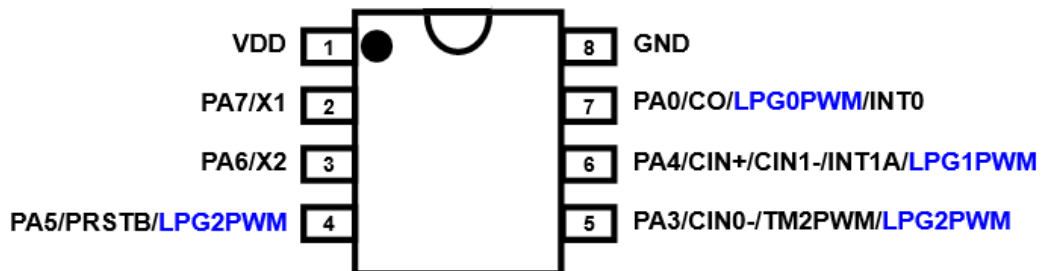
PMS152G-S08 (SOP8-150mil)
